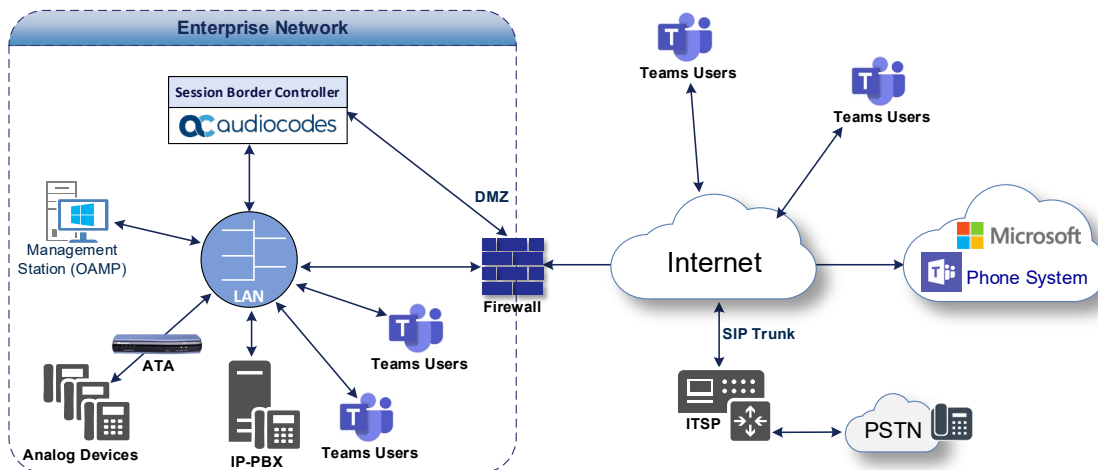
Figure 2-1: Interoperability Test Topology between SBC and Microsoft Teams Direct Routing Enterprise Model with IXICA SIP Trunk
